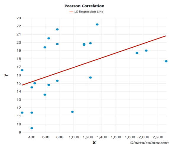
Figure 1. Correlation between the male second polar moment of area and minimum temperature in Centrobolus Cook, 1897.
