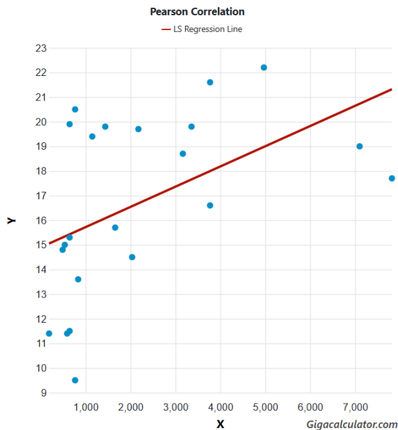
Figure 2. Correlation between the female second polar moment of area and minimum temperature in Centrobolus Cook, 1897.
