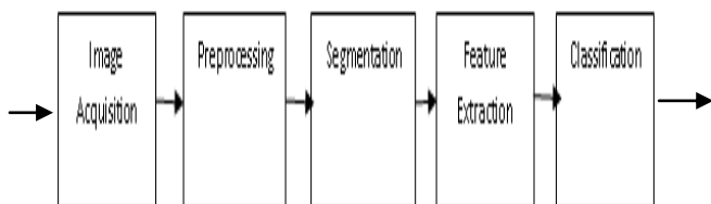
Figure 1: CAD System
