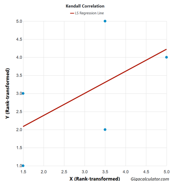
Figure 1. Correlation between the male second polar moment of area and male mass in Centrobolus Cook, 1897.
