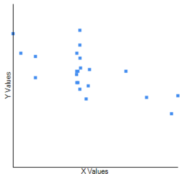
Fig. 1 Width in females correlated to highest total hours of sunshine in a month in Centrobolus Cook , 1897.
