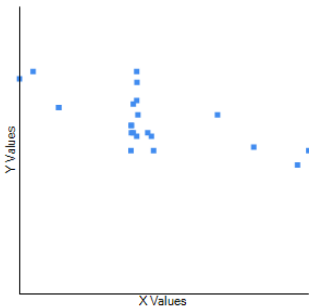
Fig. 2 Width in males marginally correlated to highest total hours of sunshine in a month in Centrobolus Cook, 1897.
