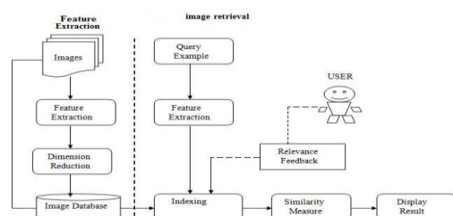
Figure 1: Content based image retrieval.
