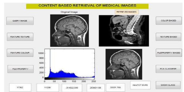
Figure3: Retrieved image of class of CT Scan Image with Histogram plot.
