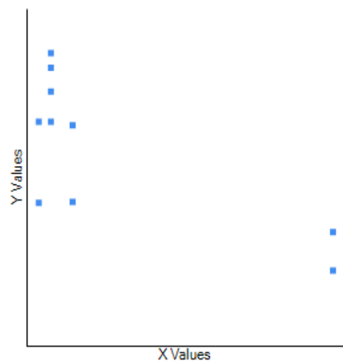
Fig. 1. Correlation between mass (Y) and lowest number of daily hours of sunshine in a day (X) across the range of Centrobolus Cook, 1897.
