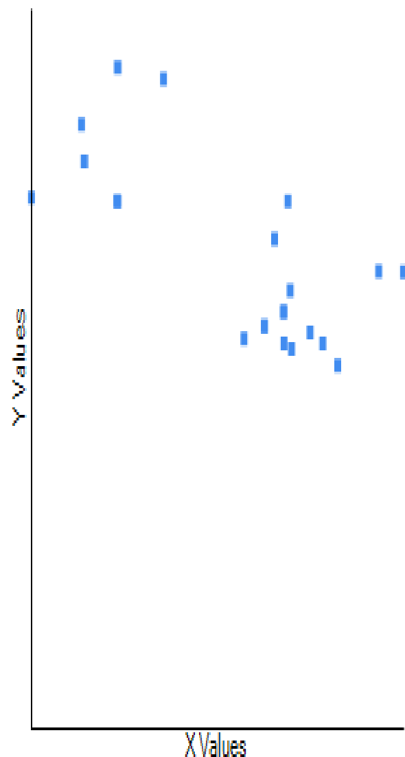
Fig. 1. Correlation between the precipitation (X) and lowest number of dailyhours of sunshine in a day (Y) across the range of Centrobolus Cook, 1897.
