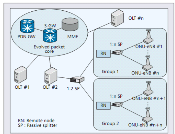
Fig. 3 Remote Node Integration Architecture(RNIA)
