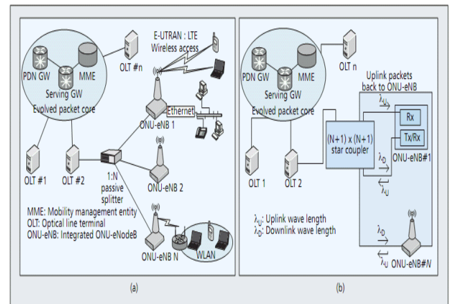
Fig.2 (a) Native-10 GEPON-LTE Integration Architecture (b) Loopback Integration Architecture
