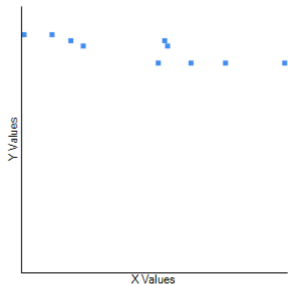
Fig. 1. Correlation between moments of inertia (X) and lowest relative humidity (Y) across the range of Centrobolus Cook, 1897.
