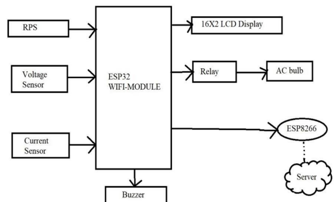
Fig 2.1 Block diagram
