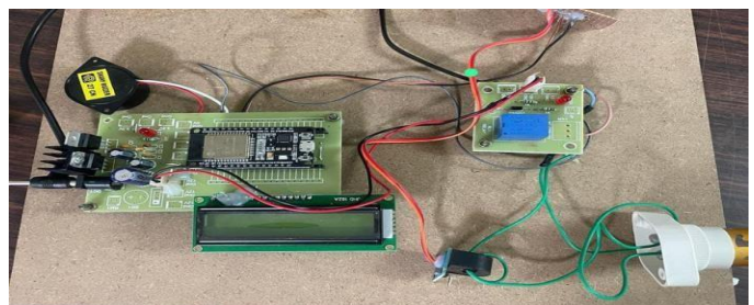
Fig 4.4: Circuit before giving regulated power supply
