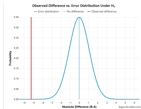
Fig. 1. Test of species richness and mean ocean water temperature across the range of Centrobolus Cook, 1897.
