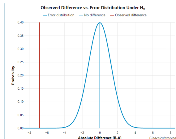
Fig. 1. P-value calculation between highest ocean water temperature and species richness in Centrobolus Cook, 1897.
