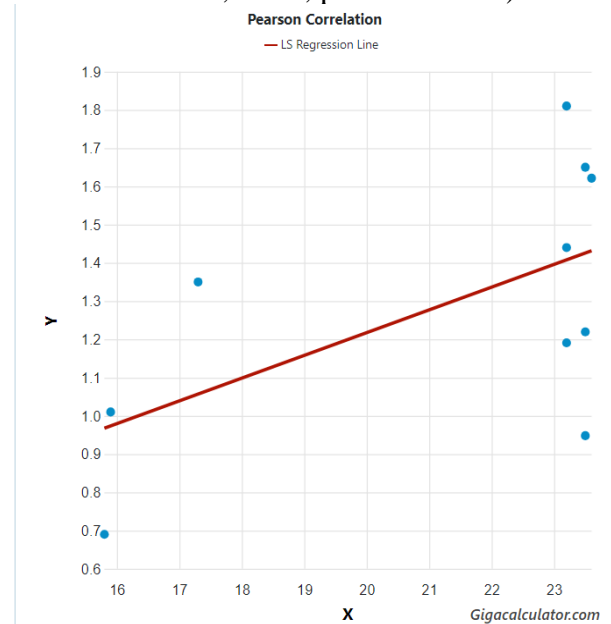
Fig. 1. Correlation between the mean ocean water temperature (x) with sexual size dimorphism (y) across the range of coastal Centrobolus Cook, 1897.
