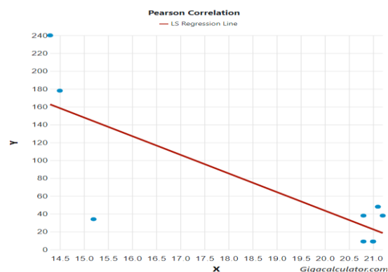
Fig. 1. Correlation between minimum ocean water temperature (X) and
