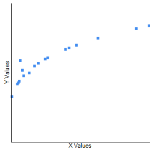
Fig. 1 Second polar moments of area correlated to female width in Centrobolus Cook, 1897.
