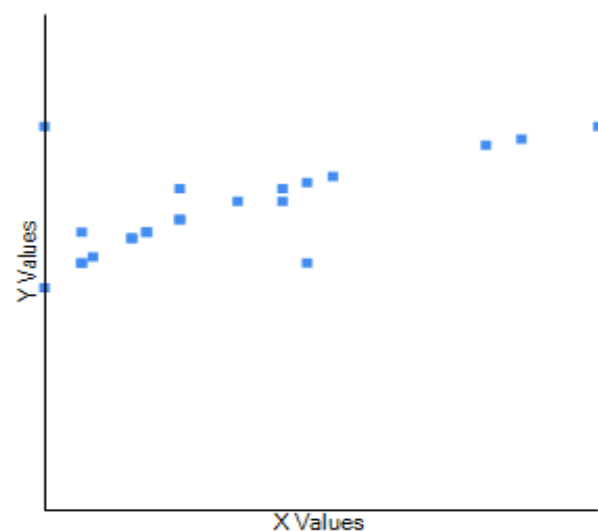
Fig. 2 Second polar moments of area correlated to male width in Centrobolus Cook, 1897.
