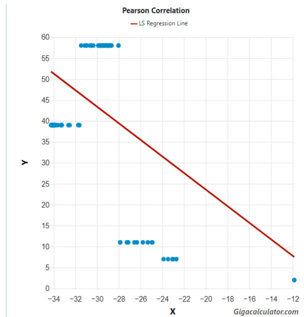
Fig. 1. Correlation between latitude (x) and species richness (y) across the range of Dalodesmidae Cook, 1896a.
