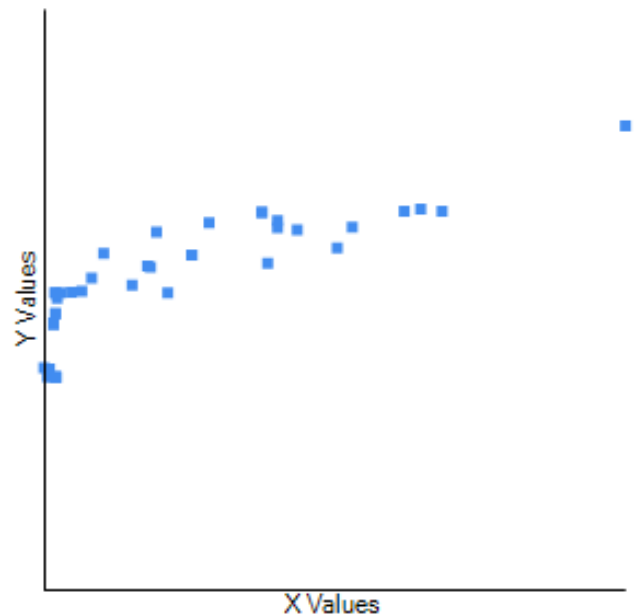
Fig. 1. Correlation between latitude (x) and longitude (y) across the range of Sphaerotherium Brandt, 1833.
