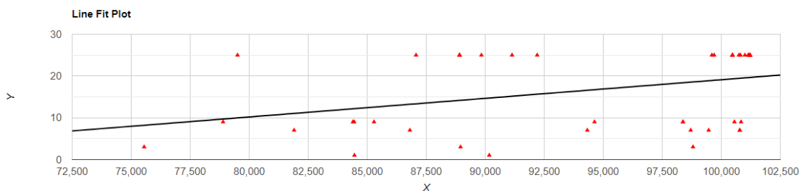
Fig. 1. Correlation between latitudinal species richness (Y) and air pressure (X) across the range of Sphaerotherium Brandt, 1833.
