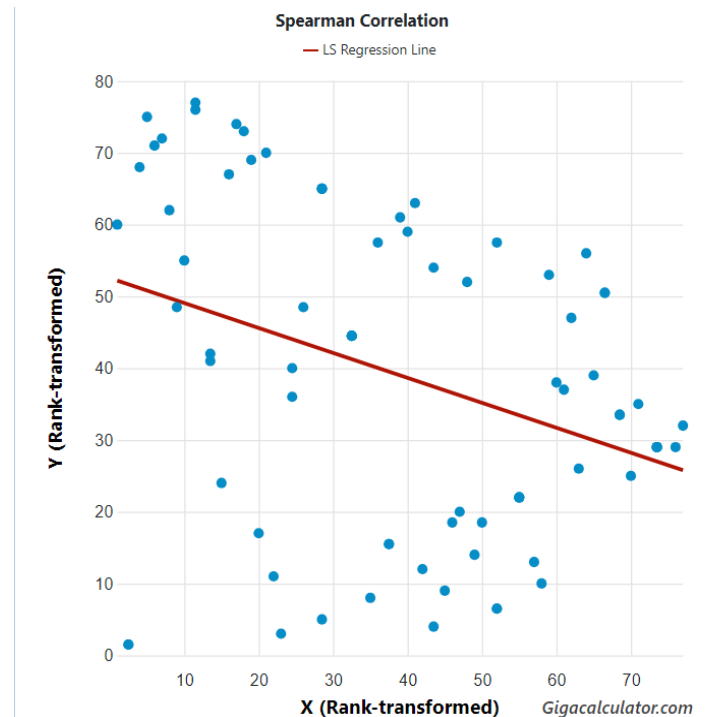
Fig. 1. Correlation between latitude (Y) and air pressure (X) across the genus of southern African keeled millipedes Gnomeskelus Attems, 1926.
