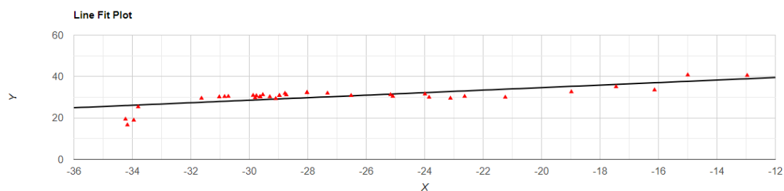
Figure 1. Correlation between latitude (x) and longitude (y) in southern African Gomphodesmidae.
