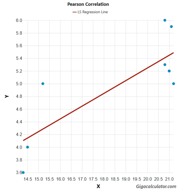
Fig. 1. Correlation between minimum ocean water temperature (x) and male width (y) across the range of Centrobolus Cook, 1897.
