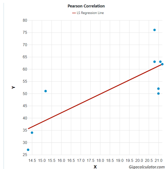
Fig. 1. Correlation between minimum ocean water temperature (x) and female length (y) across the range of Centrobolus Cook, 1897.
