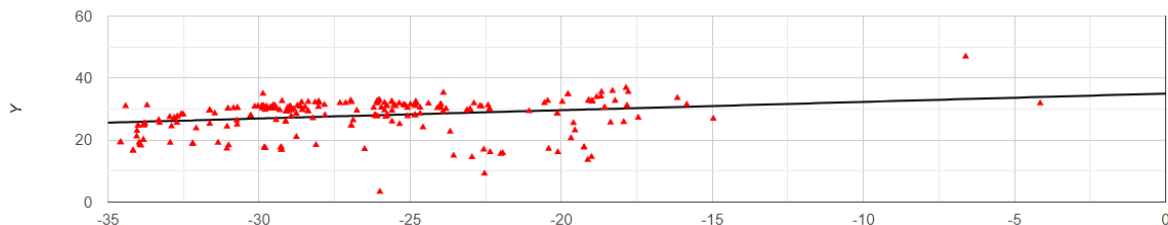
Line Fit Plot
