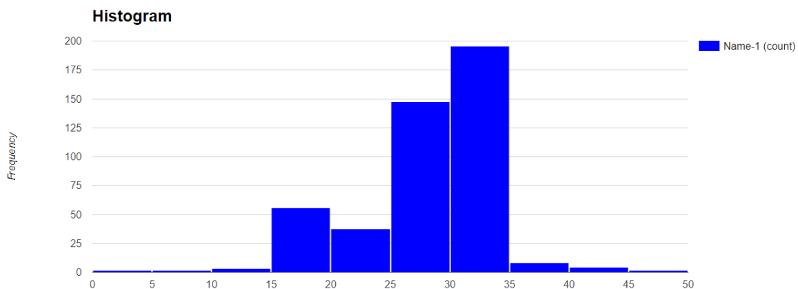
Figure 1. Longitudinal species richness in southern African Helminthomorpha Pockock, 1887.
