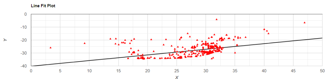
Figure 1. Correlation between latitude (y) and longitude (x) in southern African Chilognatha Latreille, 1802/1803.
