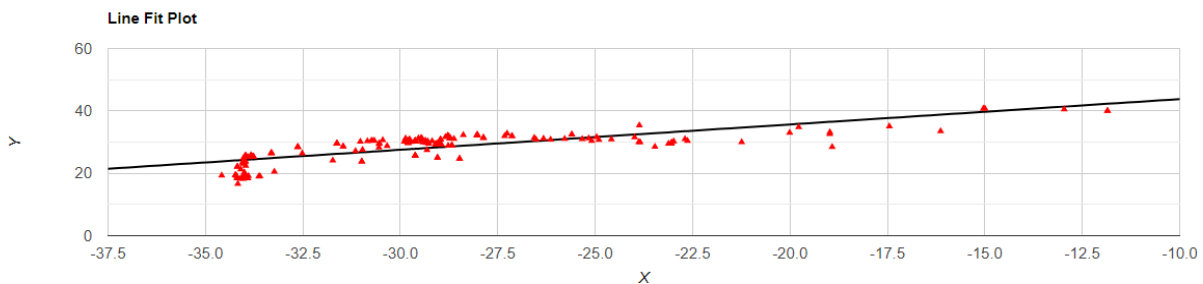
Figure 1. Latitude correlated with longitude in southern African Juliformia Attems, 1926.
