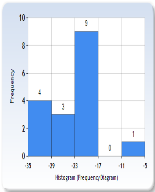
Figure 2. Histogram showing latitudinal species richness in the southern African Paradoxosomatidae Dady, 1889.
