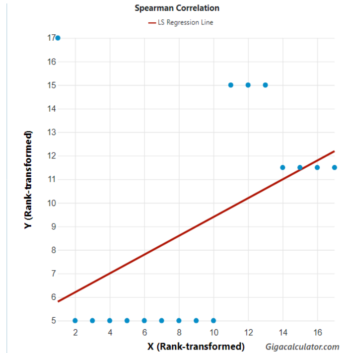
Figure 1. Correlation between latitude and species richness in the southern African Paradoxosomatidae Dady, 1889.
