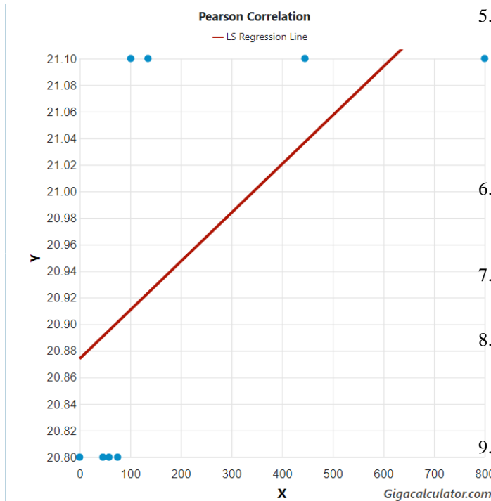
Fig. 1. Correlation between minimum ocean water temperature and abundances in Centrobolus Cook, 1897.
