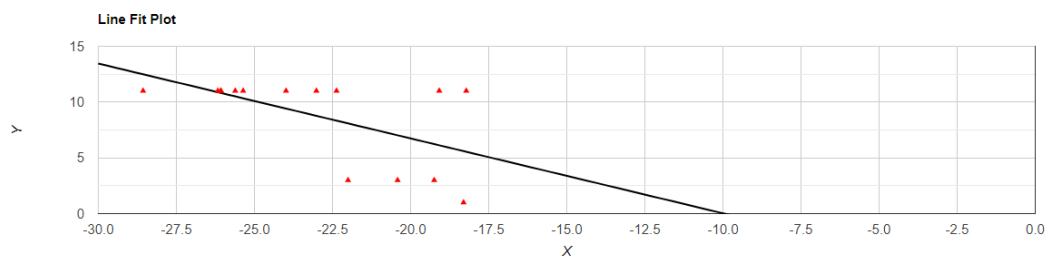
Figure 1. Longitudinal species richness correlated with latitude in southern African Patinatius Attems 1928.
