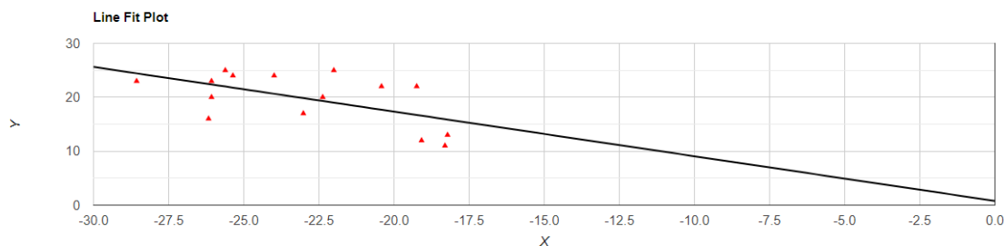
Figure 1. Correlation between temperature (x) and latitude(y) in southern African Patinatius Attems, 1928.
