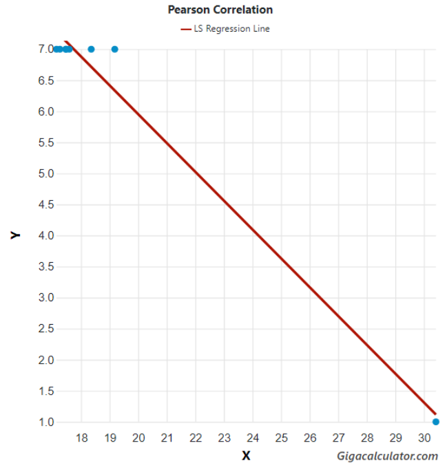
Figure 1. Longitude correlated with species richness in southern African Harpagophora Attems, 1909.
