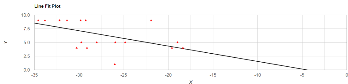
Figure 1. Longitudinal species richness correlated to latitude in southern African Chaleponcus Attems 1914b.
