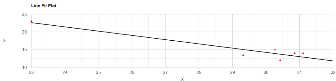
Figure 1. Temperature and longitude were correlated in southern African Phygoxerotes Verhoeff, 1939a.
